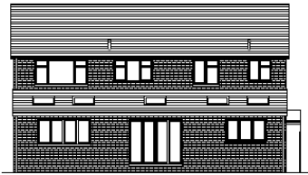
REAR ELEVATION
