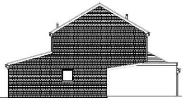
SIDE ELEVATION
